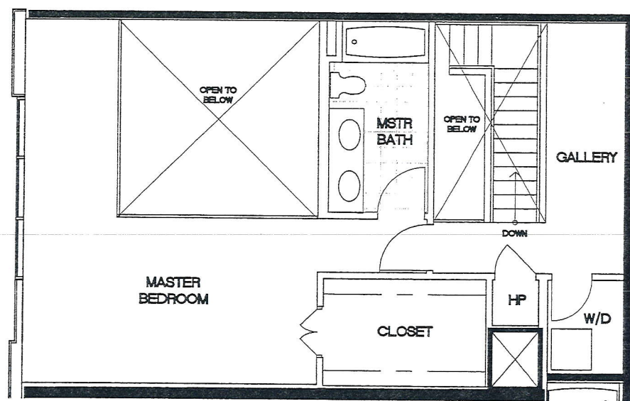
UPPER LEVEL (LEVEL 4)
